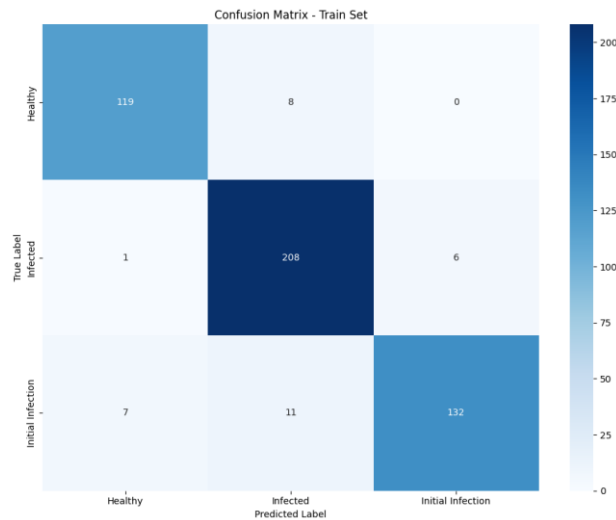
Gambar 4. Confusion Matrix (Train)
