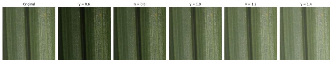
Gambar 3. Gamma Correction
