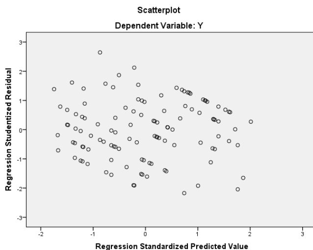
Gambar: 2 scatterplot
