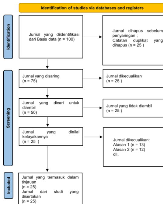
Gambar 1. Flowchart PRISMA
